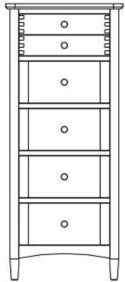
5 DRAWER WELLINGTON CHEST H: 1180 W: 550 D: 450
