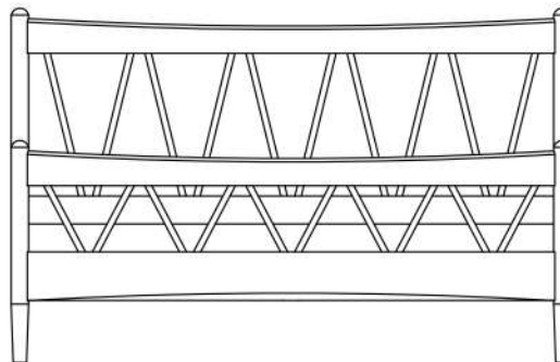
4'6" HIGH FOOT END BED H: 1020 W: 1450 D: 2003 5'0" HIGH FOOT END BED H: 1020 W: 1600 D: 2003
